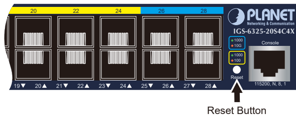
Figure 6-2: IGS-6325-20S4C4X Reset Button
